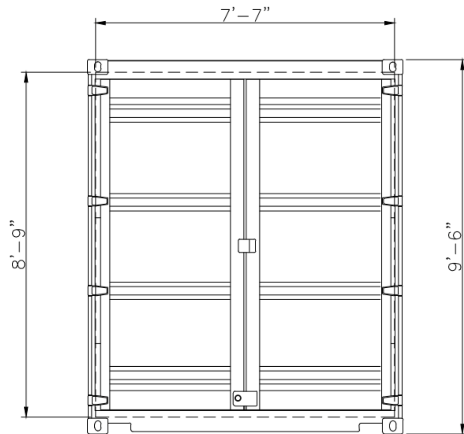
ELEVATION VIEW
